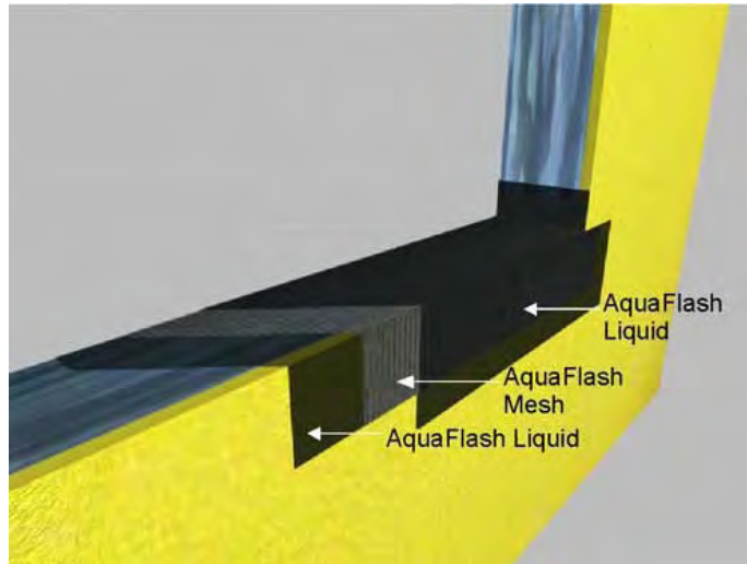
AquaFlash Liquid is applied to the substrate surface, AquaFlash Mesh is laid into it and additional AquaFlash Liquid applied over it.
