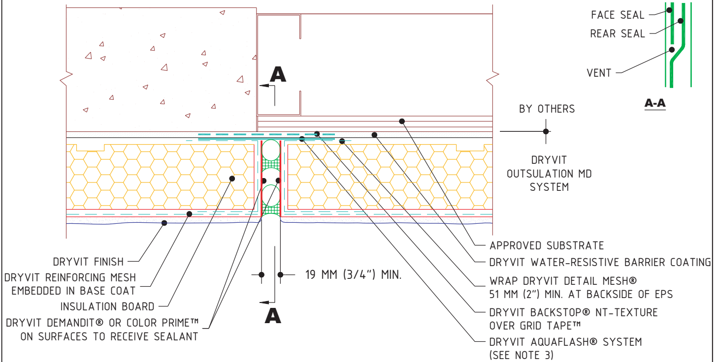
OPTION A RECESSED SEALANT
