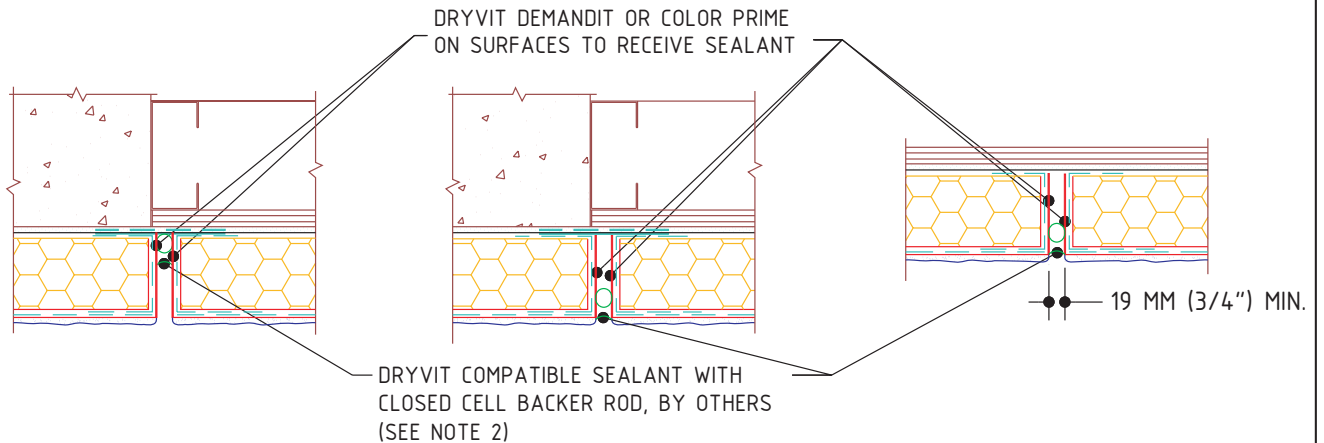
OPTION A RECESSED SEALANT
