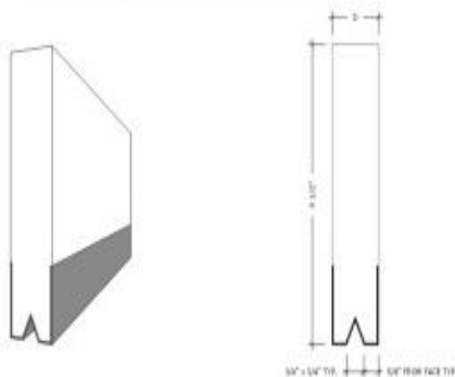
STARTER BOARD WITH DRIP EDGE
