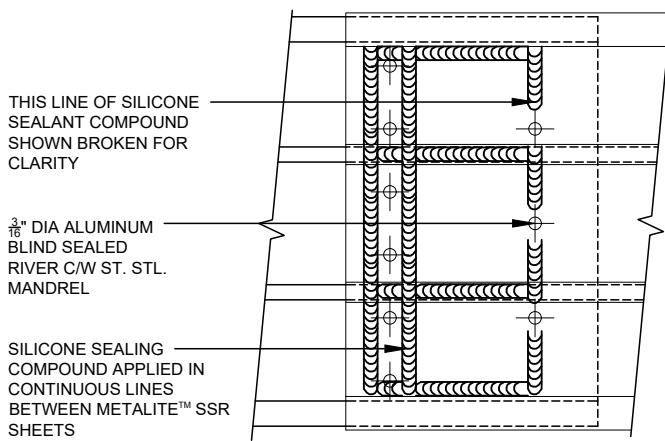
DOUBLE SKIN
