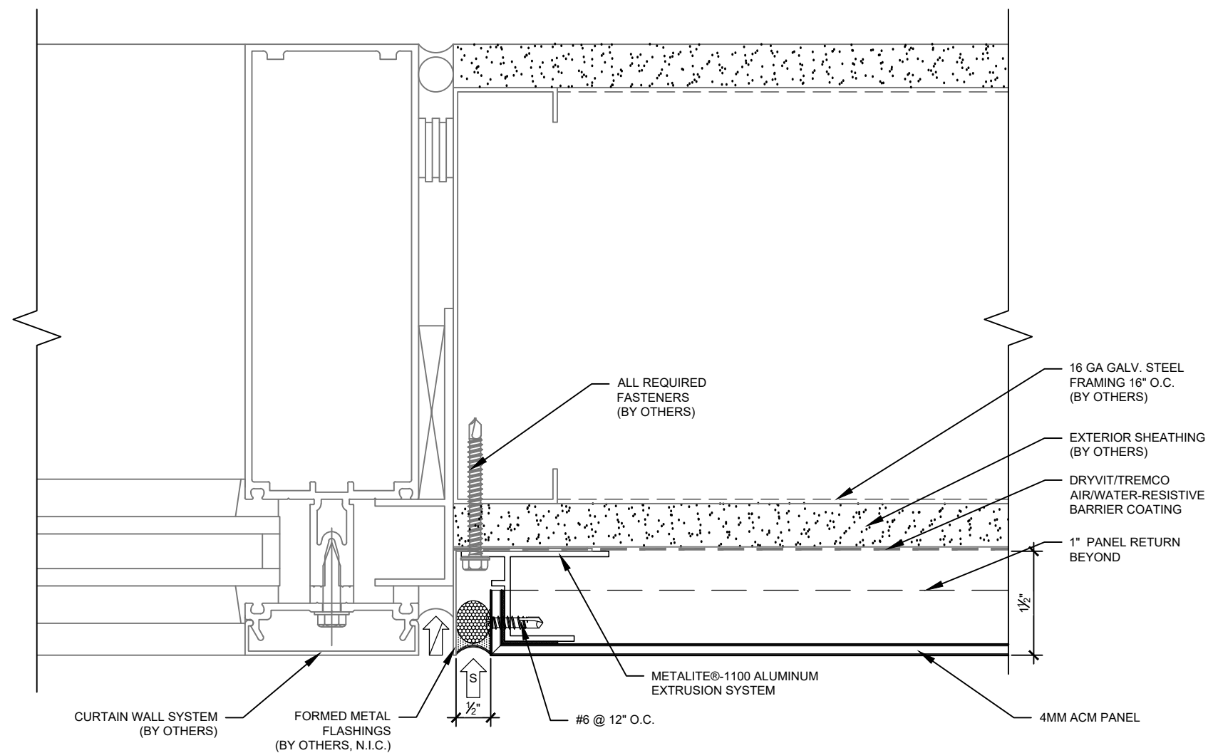
2 D.7 WINDOW JAMB DETAIL SCALE: HALF SCALE REF. ARCH.: N/A
