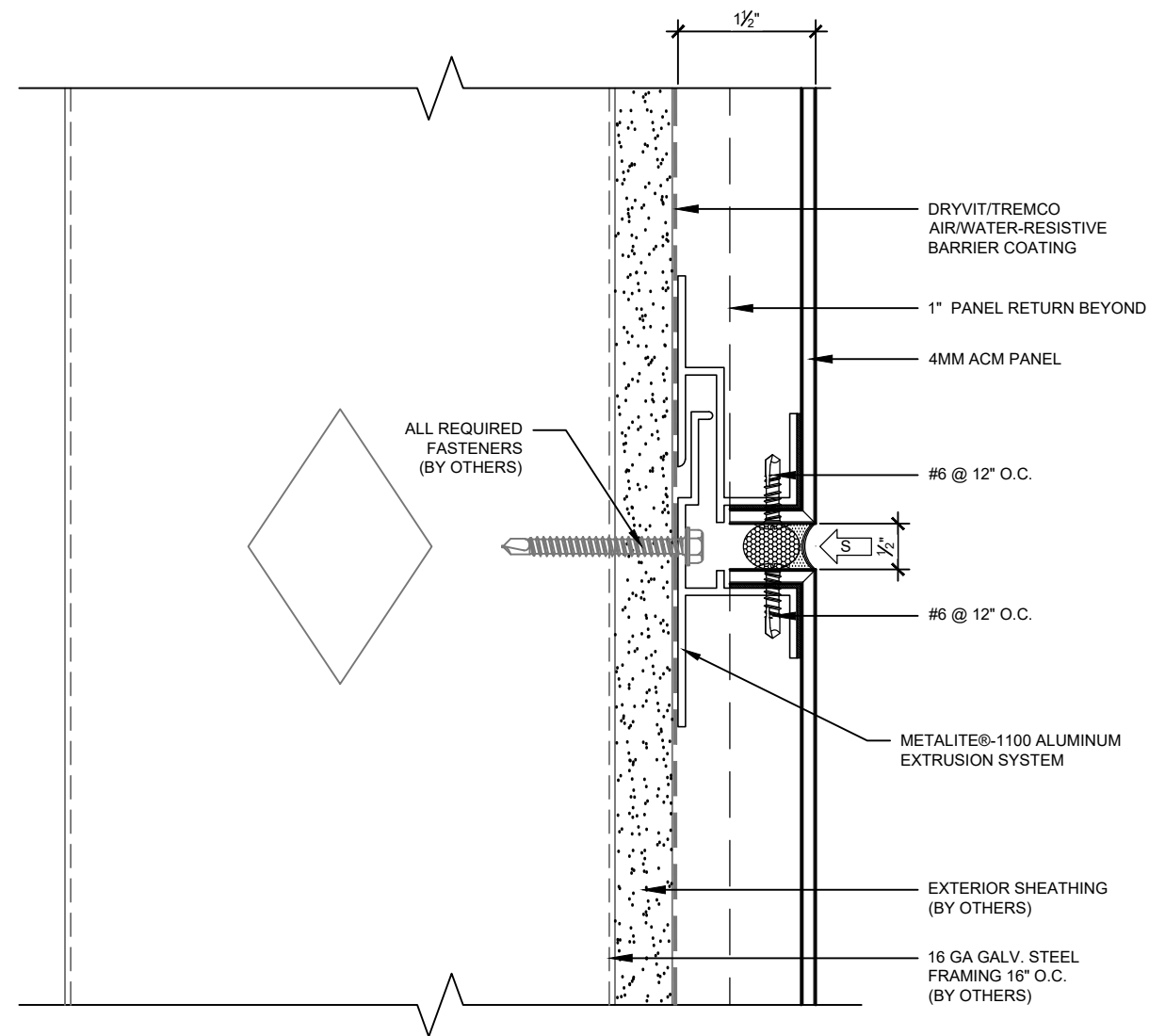
2 D.1 TYP. HORIZONTAL JOINT DETAIL SCALE: HALF SCALE REF. ARCH.: N/A
