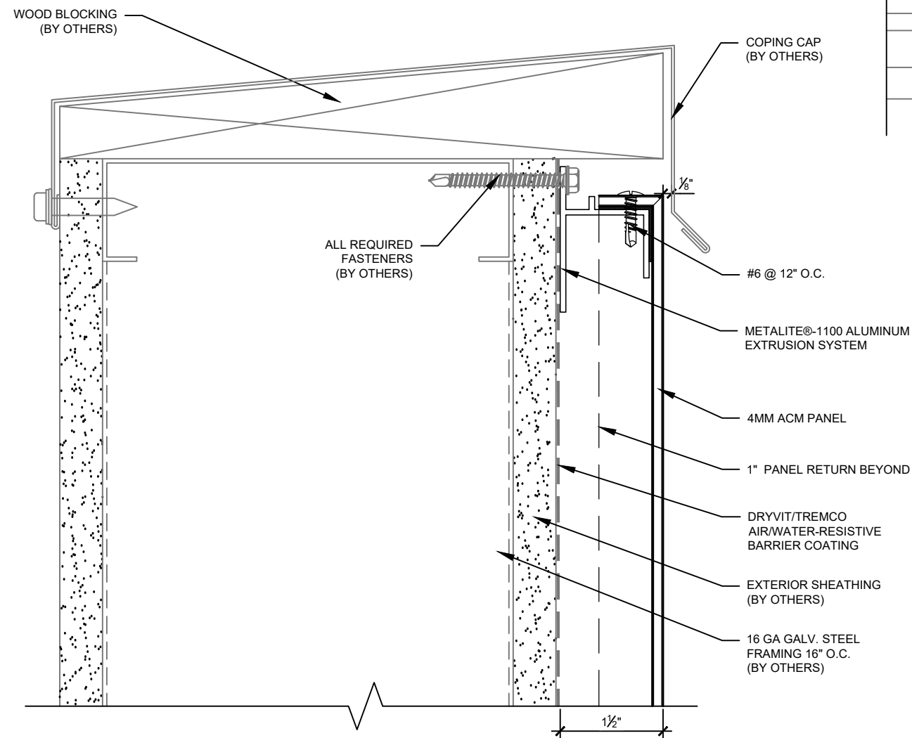
1 D.7 COPING DETAIL SCALE: HALF SCALE REF. ARCH.: N/A
