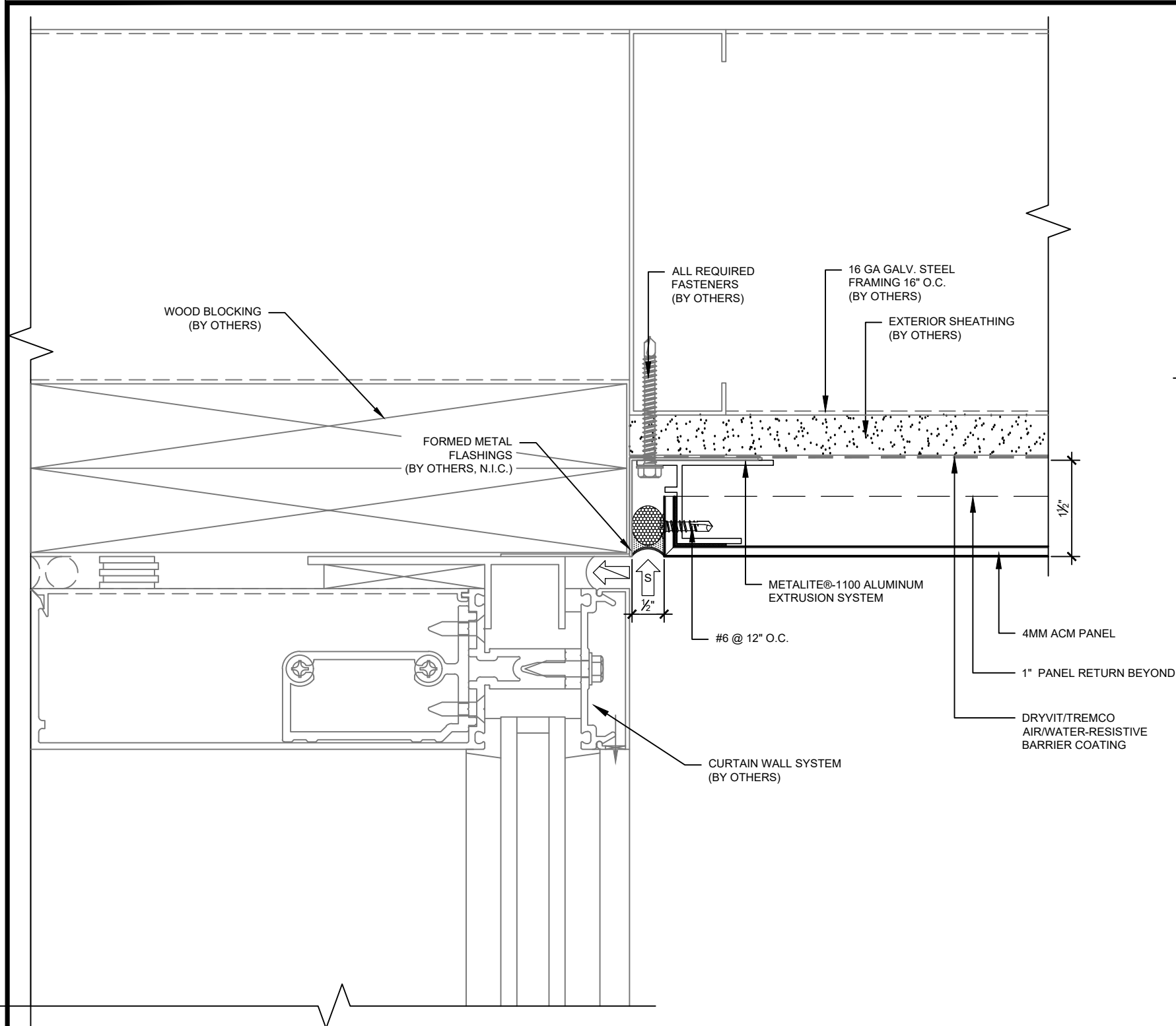
1 D.8 WINDOW HEAD/JAMB DETAIL SCALE: HALF SCALE REF. ARCH.: N/A
