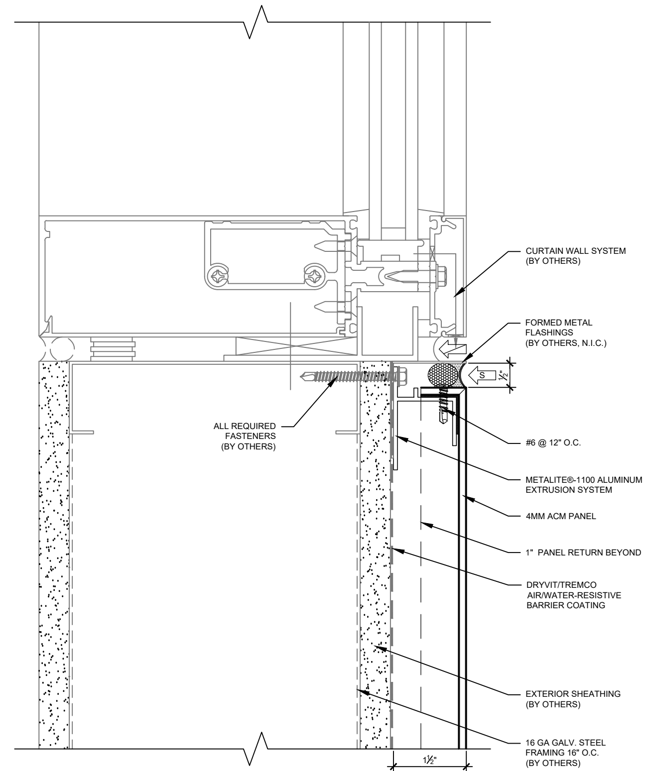
2 WINDOW SILL DETAIL SCALE: HALF SCALE REF. ARCH.: N/A
