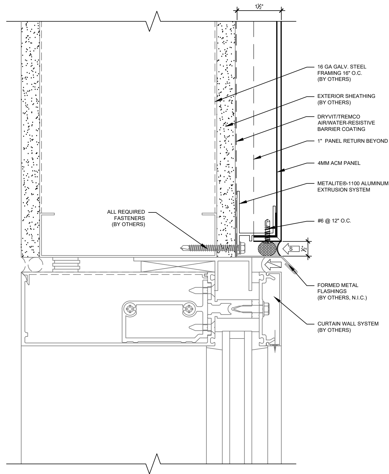
1 WINDOW HEAD DETAIL SCALE: HALF SCALE REF. ARCH.: N/A
