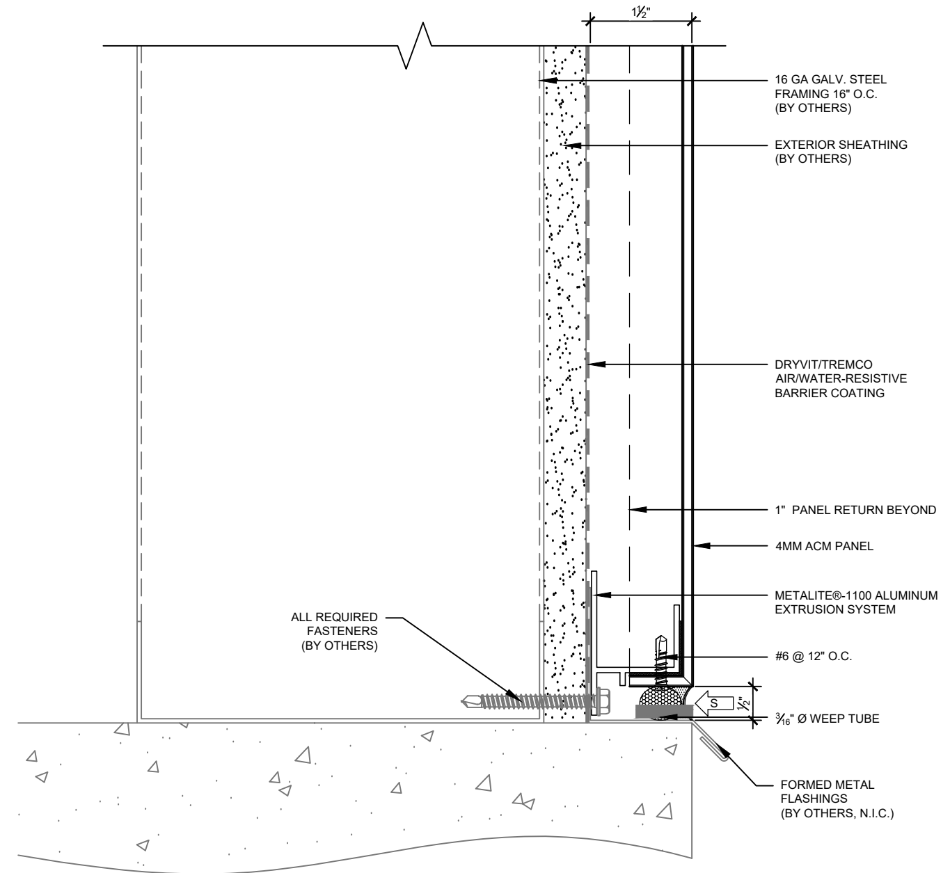
2 D.2 TYP. BASE DETAIL SCALE: HALF SCALE REF. ARCH.: N/A
