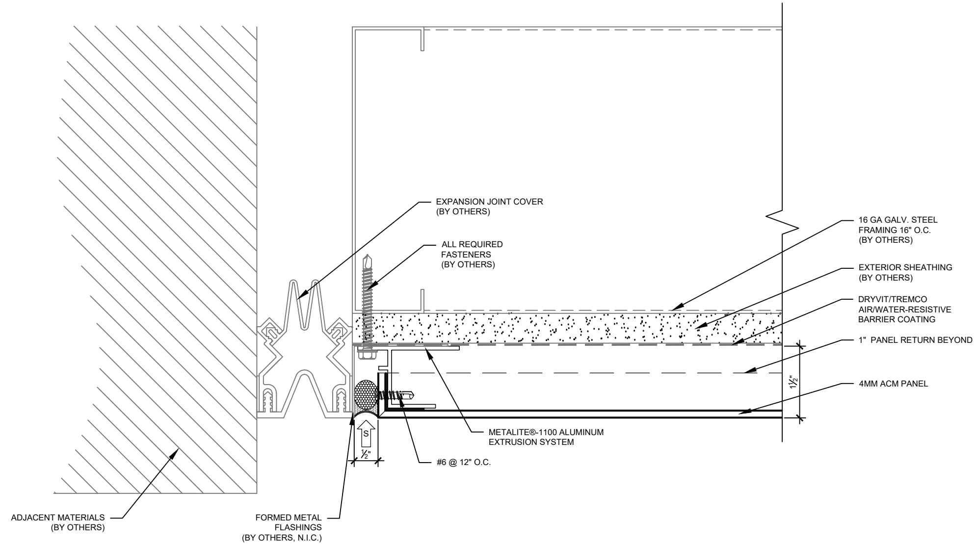
1 D.9 EXPANSION JOINT DETAIL SCALE: HALF SCALE REF. ARCH.: N/A
