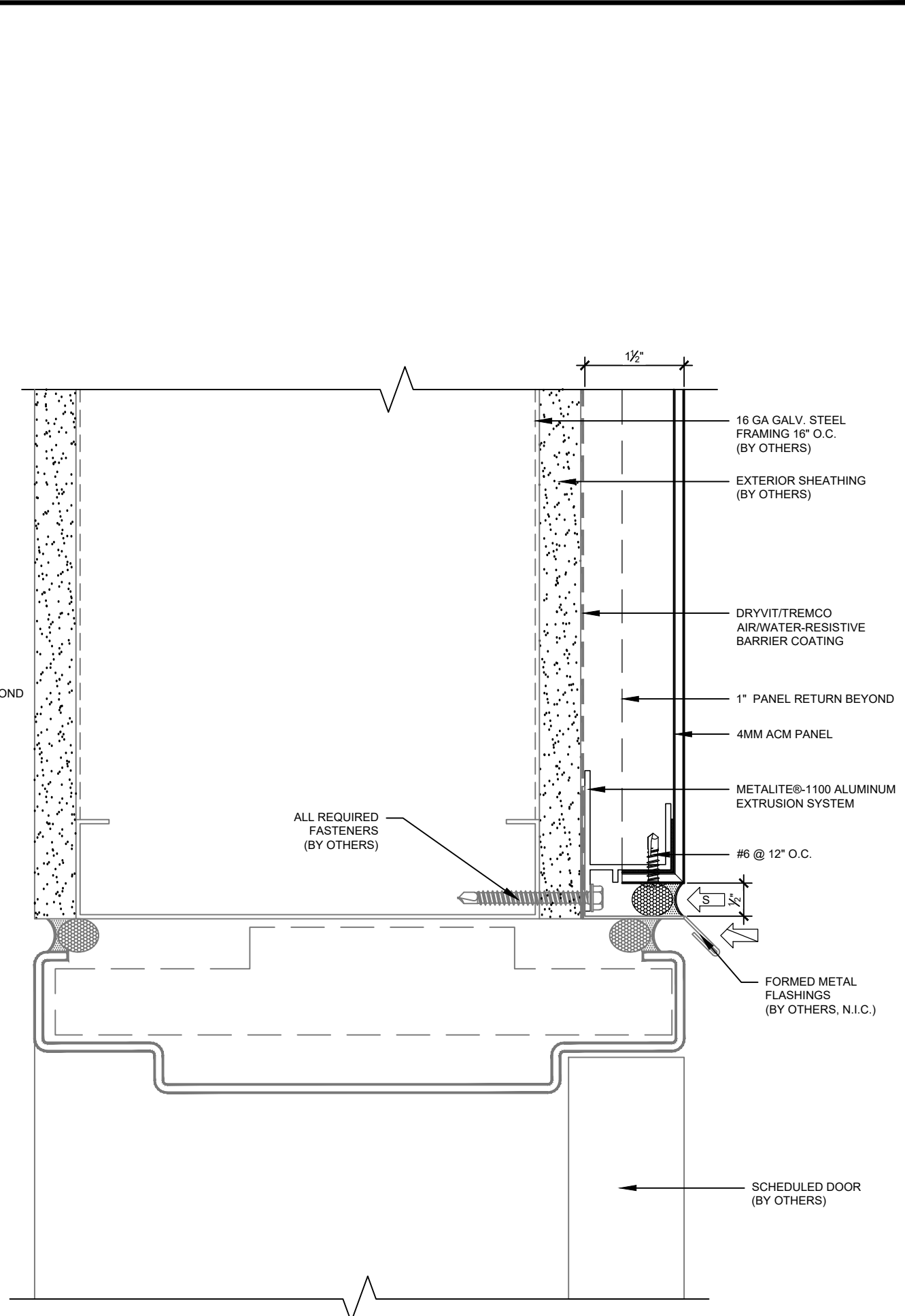
2 D.8 DOOR HEAD DETAIL SCALE: HALF SCALE REF. ARCH.: N/A
